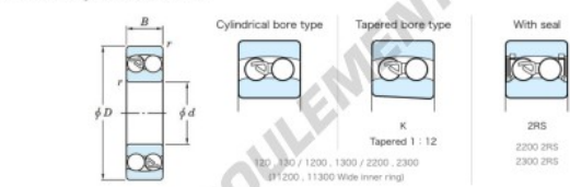
Boundary dimensions
