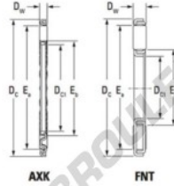
Boundary dimensions
