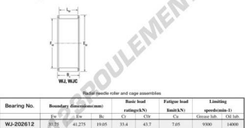
Boundary dimensions
