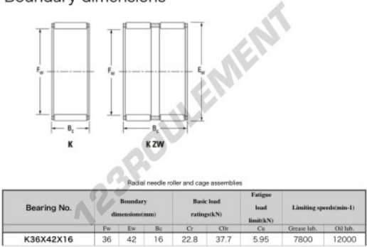
Boundary dimensions
