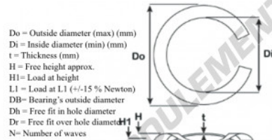
Split Wave Spring Washers
